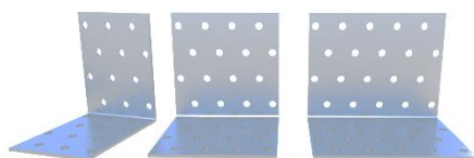
FLG 80x80x2,5x60 Cod.390406080803
